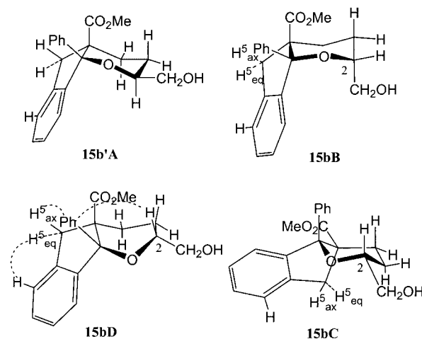
Figure 4. Conformational structures of 15b and 15b'
