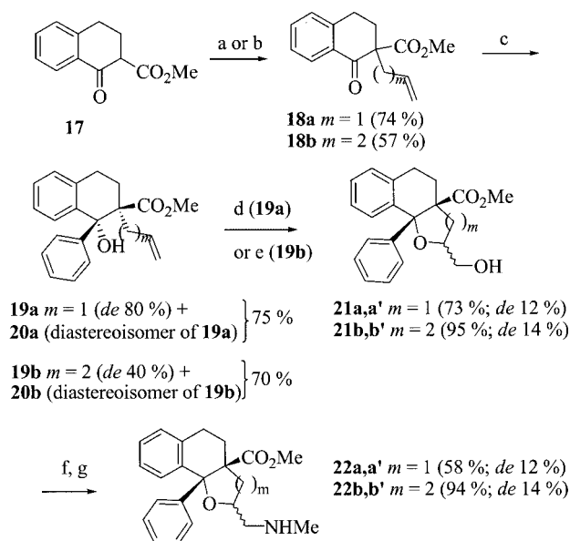
Scheme 3. Reagents and conditions: (a) NaH, 3-bromo-1-propene, DMF, 70 °C; (b) NaH, 4-bromo-1-butene, DMF, 70 °C; (c) PhMgBr, THF, -78 °C; (d) m CPBA, CH_2Cl_2 ; (e) m CPBA, CH_2Cl_2 ; then p TSA, CH_2Cl_2 ; (f) Et 3 N, MsCl, DMAP, CH_2Cl_2 , 0 °C; (g) MeNH 2 , H 2 O, 120 °C, steel bomb
