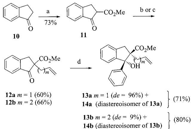
Scheme 1. Reagents and conditions: (a) NaH, (CH_3O)_2CO , reflux; (b) NaH, 3-bromo-1-propene, THF, 0 °C; (c) NaH, 4-bromo-1-butene, DMF, 70 °C; (d) PhMgBr, THF, -78 °C
